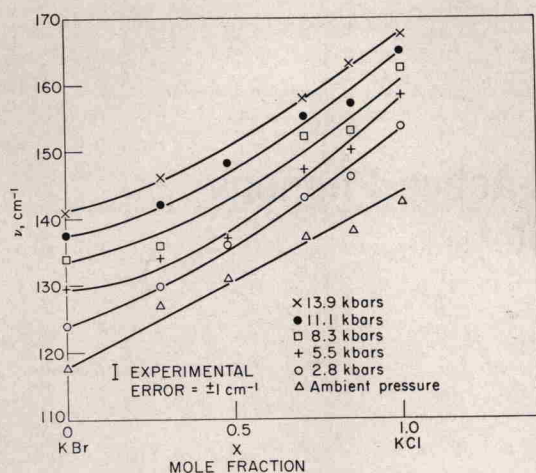
Fig. 1. Variation of the frequency of the TO mode in \text{KCl}_{1-x}\text{Br}_x system with mole fraction at various pressures.
